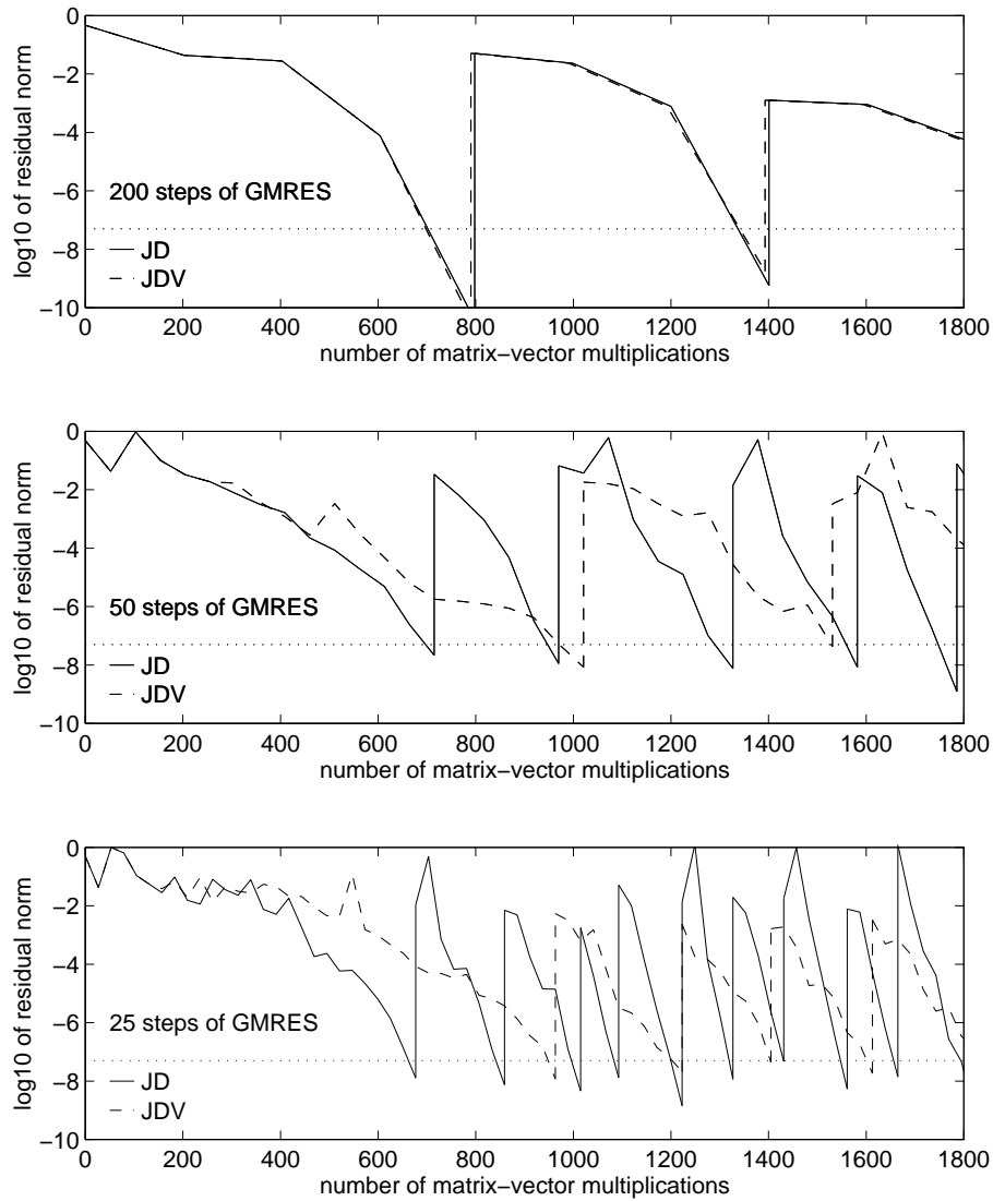
FIGURE 3. The effect of diminishing the precision of the solution method for the correction equation. Convergence plots for matrix SHERMAN1 shifted by -2.5 . The correction equation is solved with 200, 50 and 25 steps of GMRES. The plots show the \log_{10} of the residual norms for JD (the solid curve) and JDV (the dashed curve) versus the number of matrix-vector multiplications.
