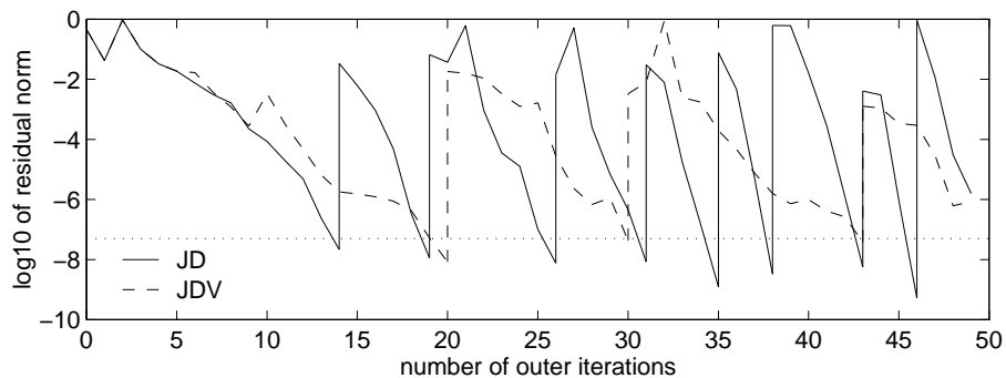
FIGURE 2. Solving the correction equation approximately with 50 steps of GMRES. Matrix SHERMAN1 shifted by -2.5 . The plot shows the \log_{10} of the residual norms for JD (solid curve) and JDV (dashed curve) versus the iteration number m .
