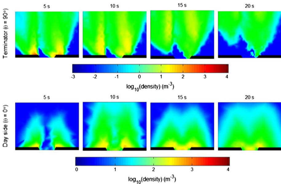
Fig. 11 Time-sequence simulations of the release of dust outside the rim of a lunar crater for two regions: terminator ( top panels ) and dayside ( bottom panels ). The crater of 5 m diameter is modelled as a opening in the bottom of the panels which represents the surface of the Moon. The x and y axes represent the lunar surface and the height of the simulation, which are 45 and 60 m, respectively
