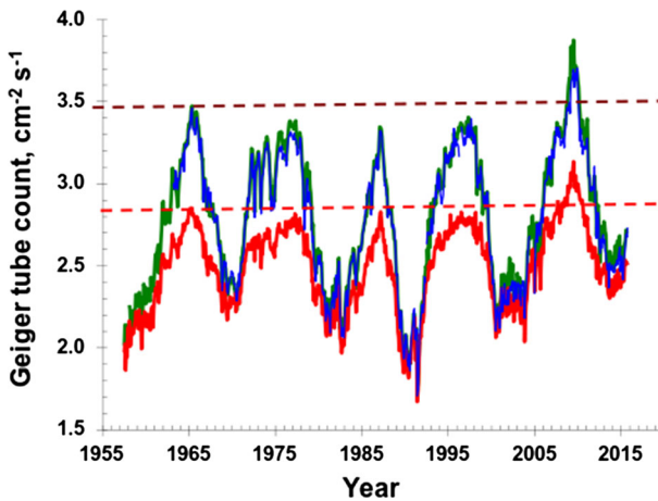
Fig. 5 Time series of monthly averages of cosmic ray fluxes, N_m [ \text{cm}^{-2} \text{s}^{-1} ], measured at the height of the Regener–Pfitzer maximum. Curves show measurements made at northern polar latitude (geomagnetic rigidity R_c = 0.6 GV, green curve), southern polar latitude in Antarctica ( R_c = 0.04 GV, blue curve) and at the midlatitude location of Moscow ( R_c = 2.4 GV, red curve). The CR flux increase since 2010 can be seen from the comparison provided by the dashed lines, which mark the cosmic ray levels in 1965 (from Stozhkov et al. 2013)
