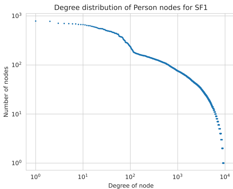
Figure 2.5: Degree distribution of the Person nodes in the SNB graph for Scale Factor 1.
