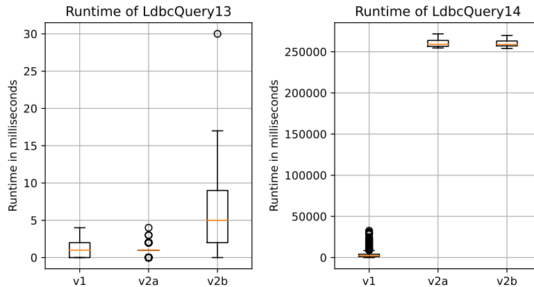
Figure 4.7: Path queries: Runtimes for path queries with interactive v1.0 and interactive v2.0 using Neo4j. Note that Q14 is changed between v1.0 and v2.0, with v2.0 performing the computationally much more difficult cheapest path problem.
