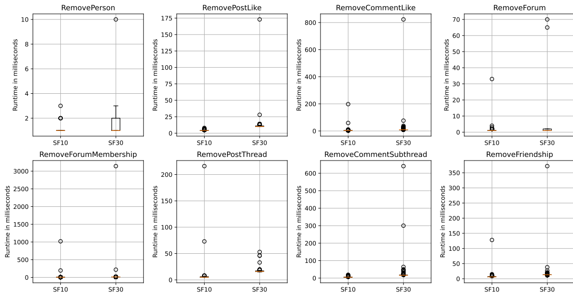
Figure 4.9: Effect of deletes: Runtimes of delete queries using Umbra for scale factors SF10 and SF30.
