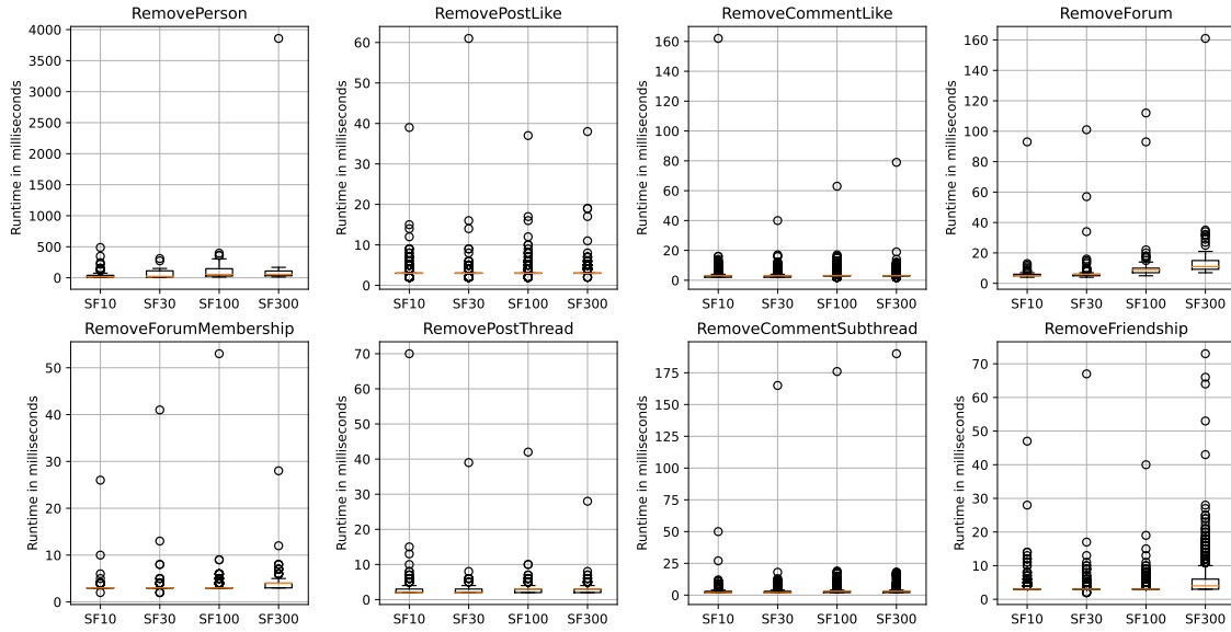
Figure 4.8: Effect of deletes: Runtimes of delete queries using Neo4j 4.4.1 for scale factors SF10, 30, 100 and 300
