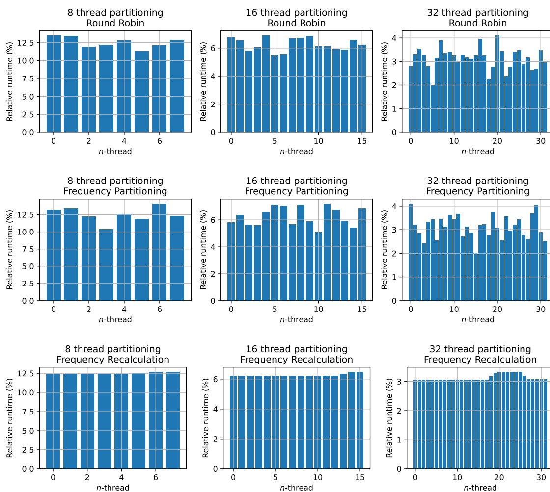
Figure 8.1: Workload distribution: relative runtimes per thread for three different partitioning strategies.
