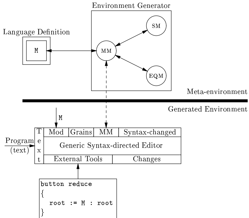
Figure 11: Generated environment for evaluating terms.
