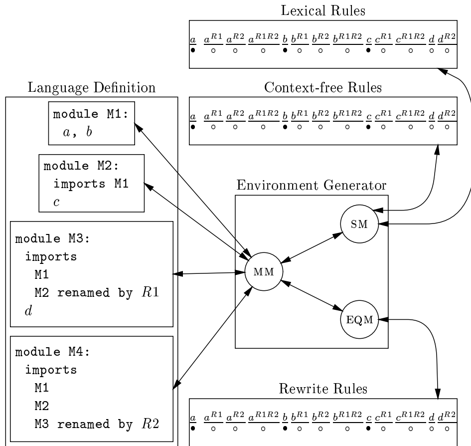
Figure 7: Processing of a modular specification (module M2 is selected)
