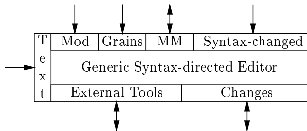
Figure 10: Generic Syntax-directed Editor (GSE) with its parameters.
