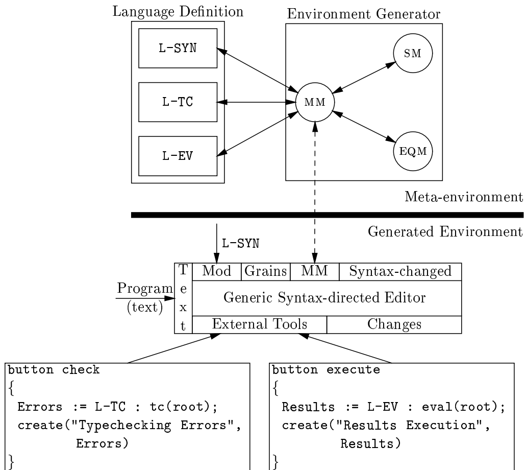
Figure 12: Generated environment for typechecking/evaluating L -programs.
