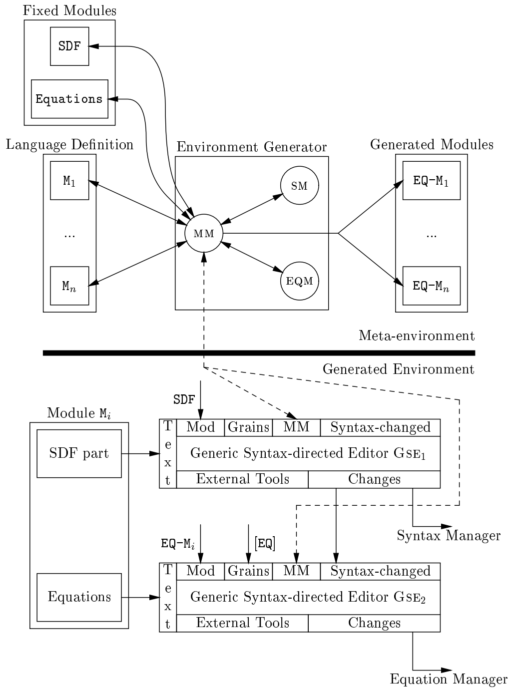
Figure 13: Editing language definition module M_i .
